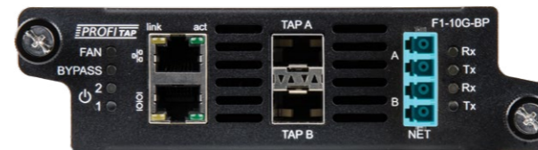
10G BYPASS TAP
