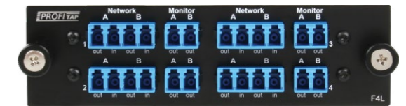
4-Link LC TAP
