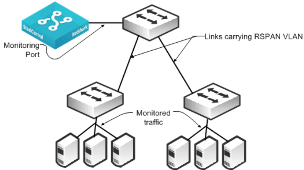
Figure 4-2. RSPAN Connectivity
